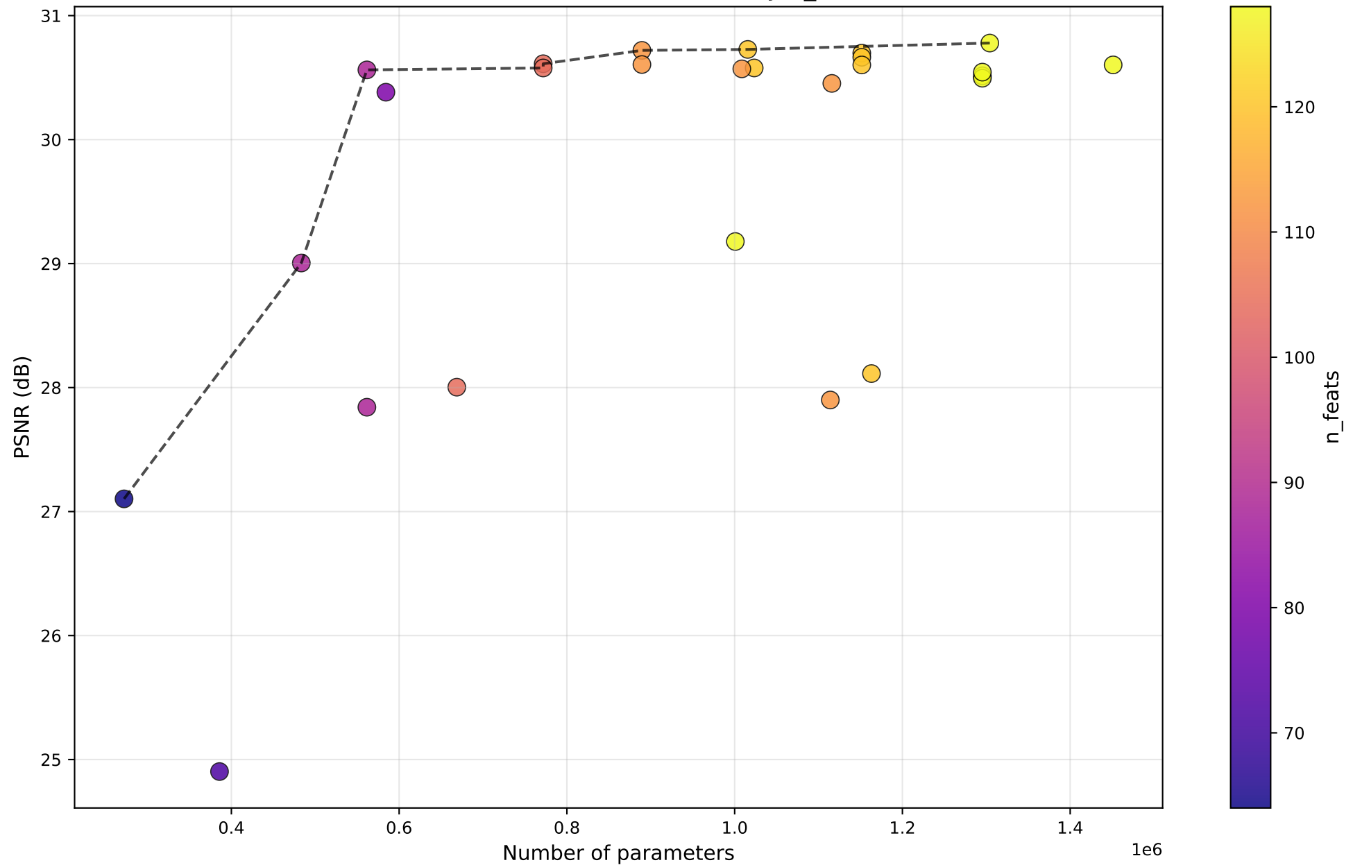
PSNR vs #Params — OmniSR — by n_feats
